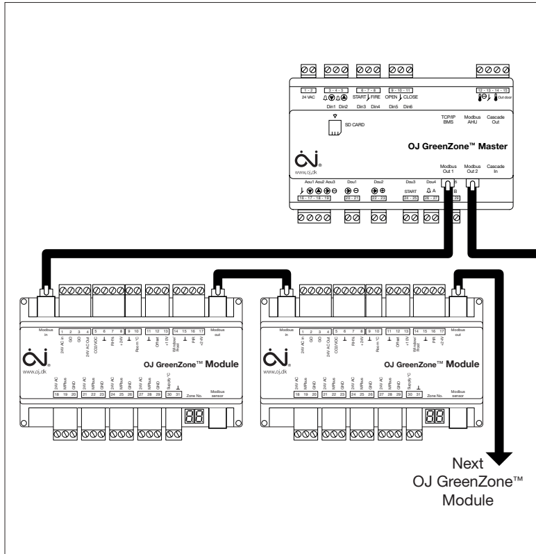
Fig. 4 - Connection of Modbus communication
