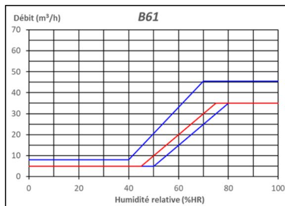
Figure 38 – B61 (5-35 m³/h, 45-75%HR)
