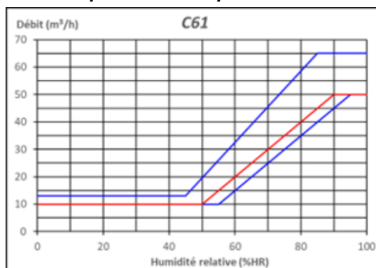
Figure 30 – C61 (10-50/75 m³/h, 50-90%HR)
