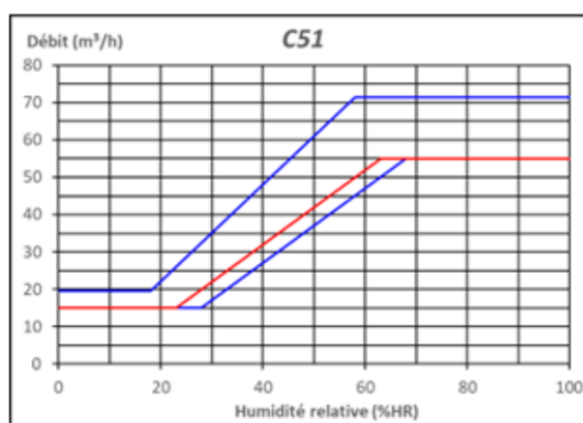
Figure 36 – C51 (15-55/135 m³/h, 23-63%HR)
