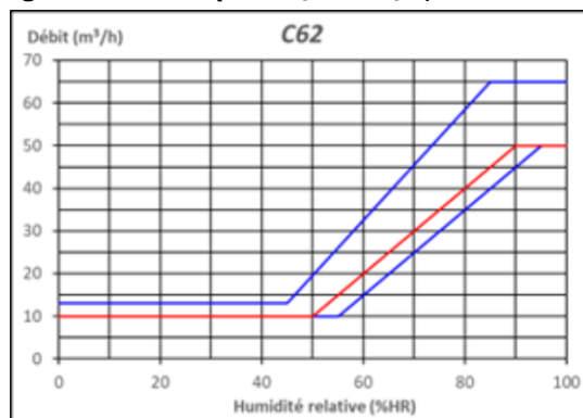
Figure 31 – C62 (10-50/90 m³/h, 50-90%HR)
