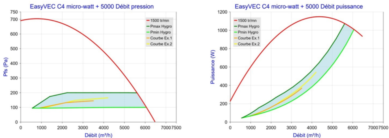
Figure 64 - EasyVEC C4 micro-watt + 5000 (sans T.Flow Hygro+/T.Flow Nano ou T.Flow 105 / T.Flow 180)
