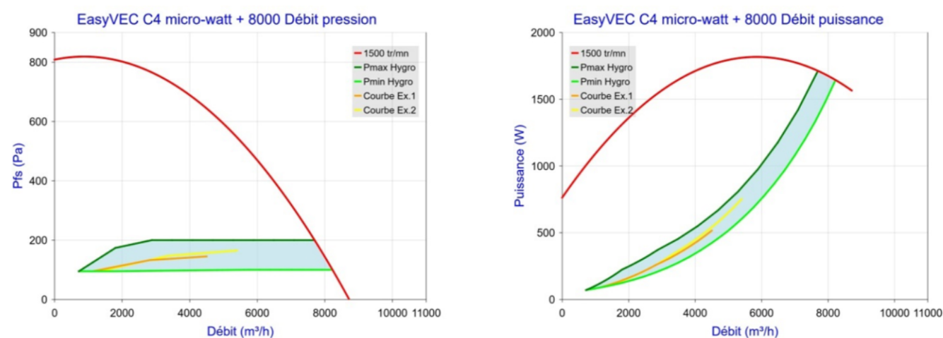
Figure 66 - EasyVEC C4 micro-watt + 8000 (sans T.Flow Hygro+/T.Flow Nano ou T.Flow 105 / T.Flow 180)
