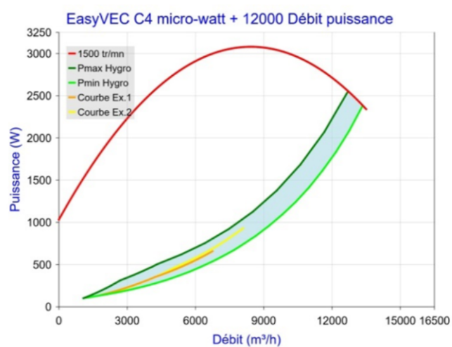
Figure 68 - EasyVEC C4 micro-watt + 12000 (sans T.Flow Hygro+/T.Flow Nano ou T.Flow 105 / T.Flow 180)
