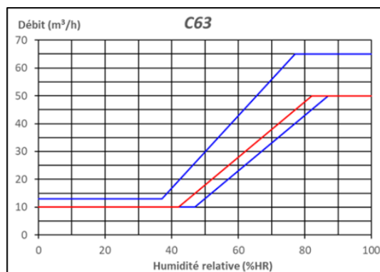
Figure 32 – C63 (10-50/105 m³/h, 42-82%HR)
