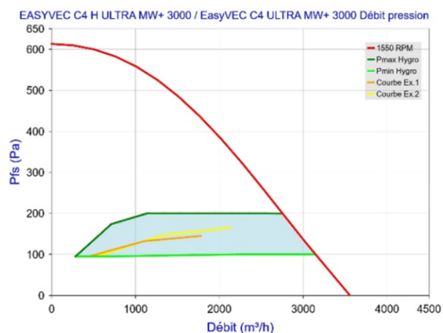
Figure 88 - EasyVEC C4 (H) ULTRA MW+ 3000 (sans T.Flow Hygro+/T.Flow Nano ou T.Flow 105 / T.Flow 180)
