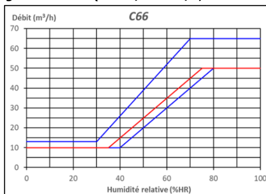
Figure 35 – C66 (10-50/90 m³/h, 35-75%HR)
