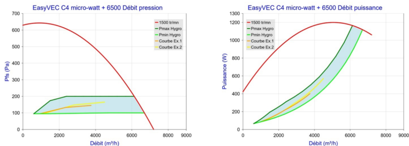
Figure 65 - EasyVEC C4 micro-watt + 6500 (sans T.Flow Hygro+/T.Flow Nano ou T.Flow 105 / T.Flow 180)
