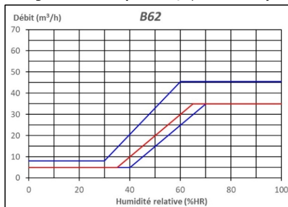
Figure 39 – B62 (5-35 m³/h, 35-65%HR)
