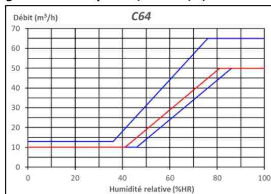
Figure 33 – C64 (10-50/120 m³/h, 41-81%HR)
