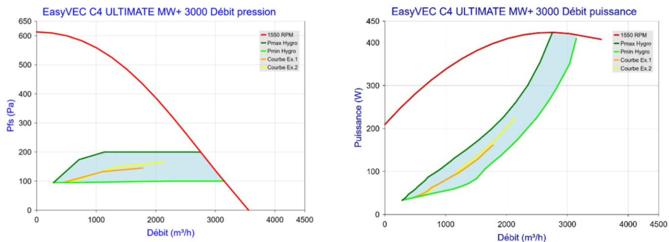
Figure 104 - EasyVEC C4 ULTIMATE MW+ 3000 (sans T.Flow Hygro+/T.Flow Nano ou T.Flow 105 / T.Flow 180)
