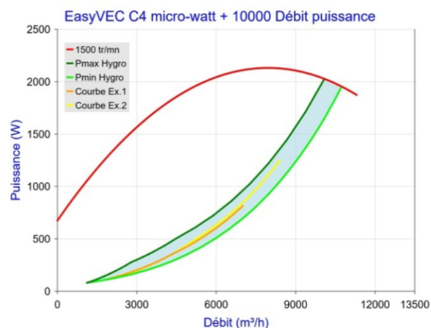
Figure 67 - EasyVEC C4 micro-watt + 10000 (sans T.Flow Hygro+/T.Flow Nano ou T.Flow 105 / T.Flow 180)
