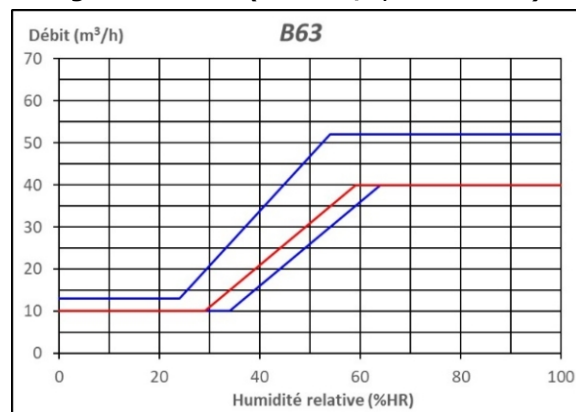
Figure 40 – B63 (10-40 m³/h, 29-59%HR)
