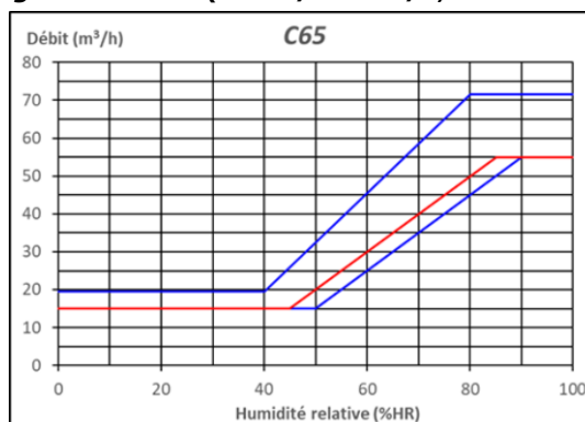
Figure 34 – C65 (15-55/135 m³/h, 45-85%HR)
