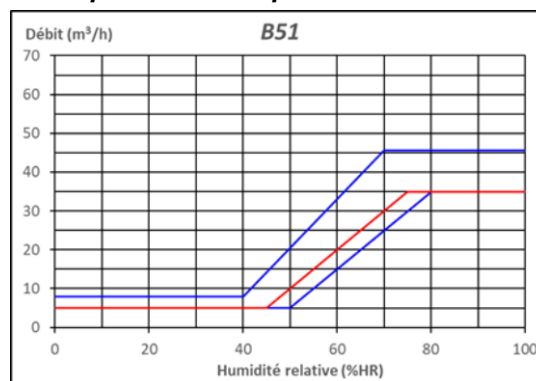
Figure 34 – B51 (5-35 m³/h, 45-75%HR)
