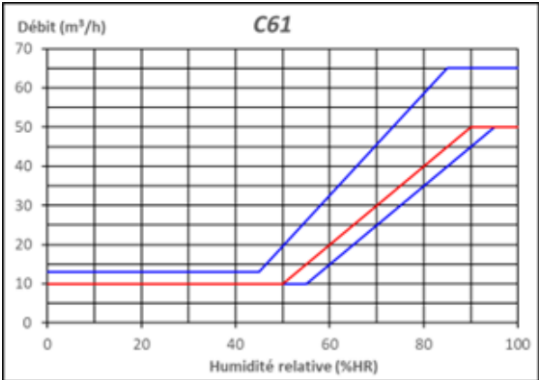
Figure 31 – C61 (10-50/75 m³/h, 50-90%HR)
