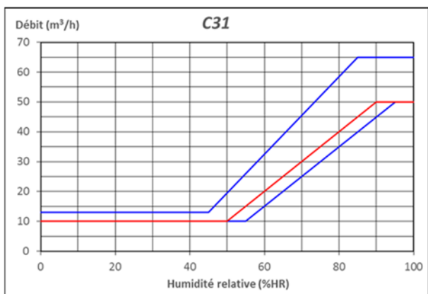
Figure 23 – C31 (10-50/75 m³/h, 50-90%HR)
