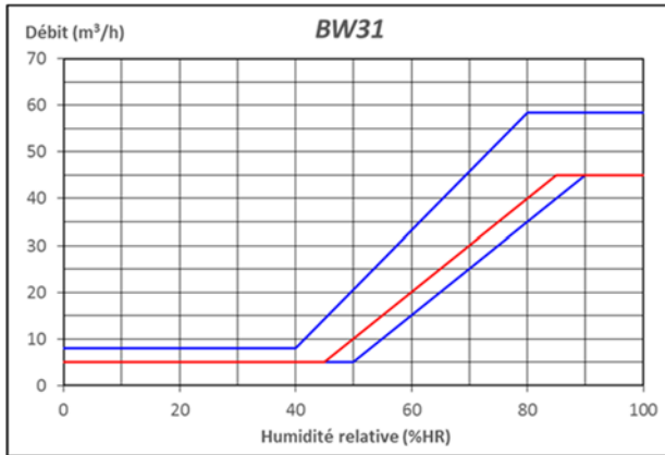
Figure 33 – BW31 (5-45/30 m³/h, 45-85%HR)
