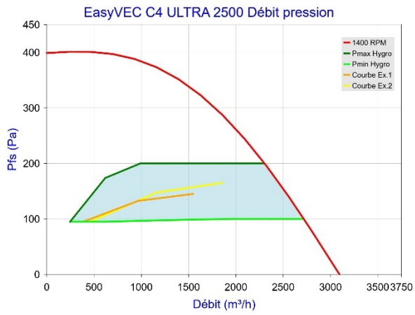
Figure 40 - EasyVEC C4 ULTRA 2500 (sans T.Flow Hygro+ /T.Flow Nano)
