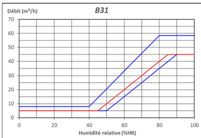
Figure 30 – B31 (5-45 m³/h, 45-85%HR)
