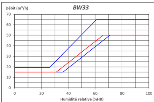
Figure 35 – BW33 (15-50/50 m³/h, 31-66%HR)
