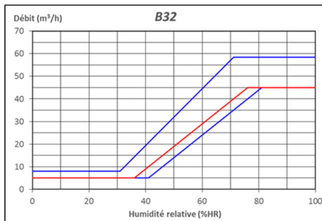
Figure 31 – B32 (5-45 m³/h, 36-76%HR)
