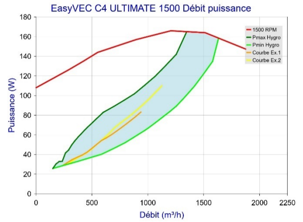
Figure 54 - EasyVEC C4 ULTIMATE 1500 (sans T.Flow Hygro+/T.Flow Nano)
