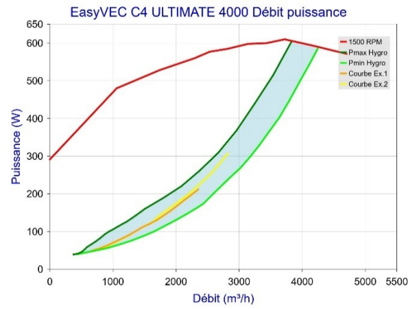
Figure 58 - EasyVEC C4 ULTIMATE 4000 (sans T.Flow Hygro+ /T.Flow Nano)
