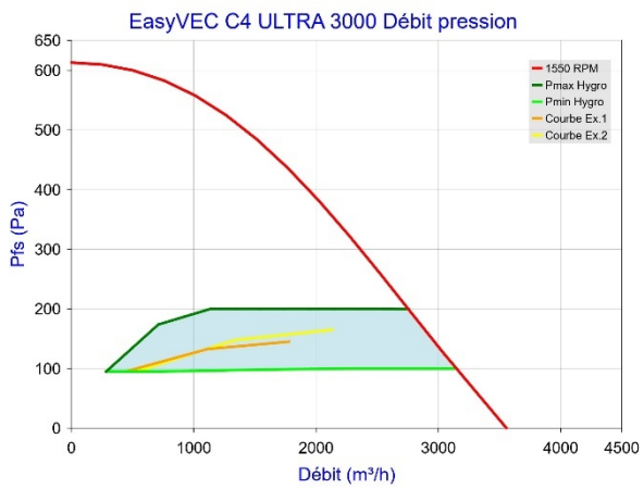
Figure 41 - EasyVEC C4 ULTRA 3000 (sans T.Flow Hygro+ /T.Flow Nano)
