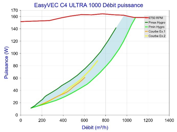
Figure 37 - EasyVEC C4 ULTRA 1000 (sans T.Flow Hygro+/T.Flow Nano)
