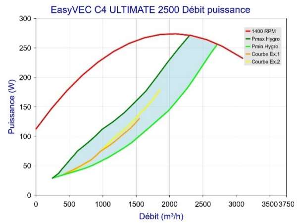
Figure 56 - EasyVEC C4 ULTIMATE 2500 (sans T.Flow Hygro+/T.Flow Nano)
