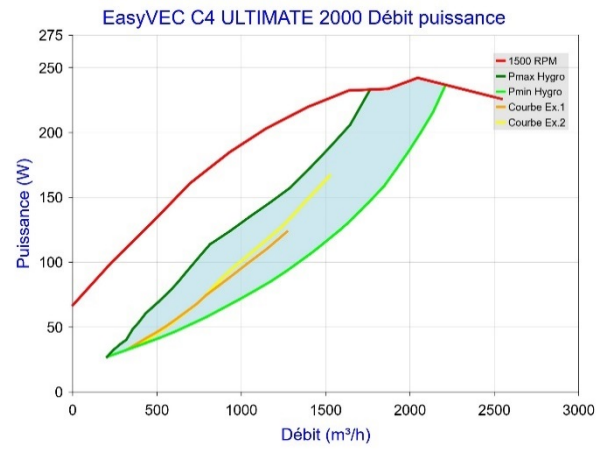
Figure 55 - EasyVEC C4 ULTIMATE 2000 (sans T.Flow Hygro+/T.Flow Nano)
