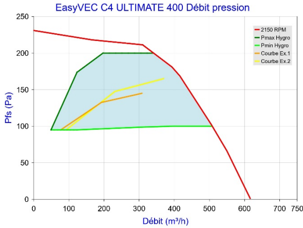
Figure 51 - EasyVEC C4 ULTIMATE 400 (sans T.Flow Hygro+ /T.Flow Nano)
