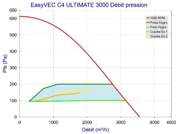
Figure 57 - EasyVEC C4 ULTIMATE 3000 (sans T.Flow Hygro+ /T.Flow Nano)
