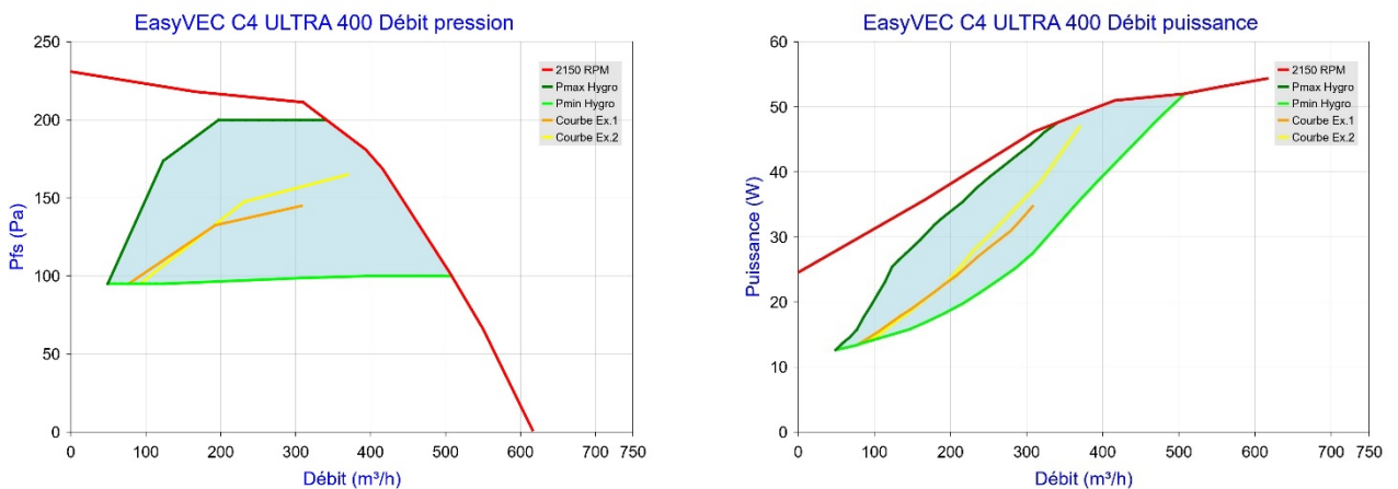
Figure 35 - EasyVEC C4 ULTRA 400 (sans T.Flow Hygro+ /T.Flow Nano)
