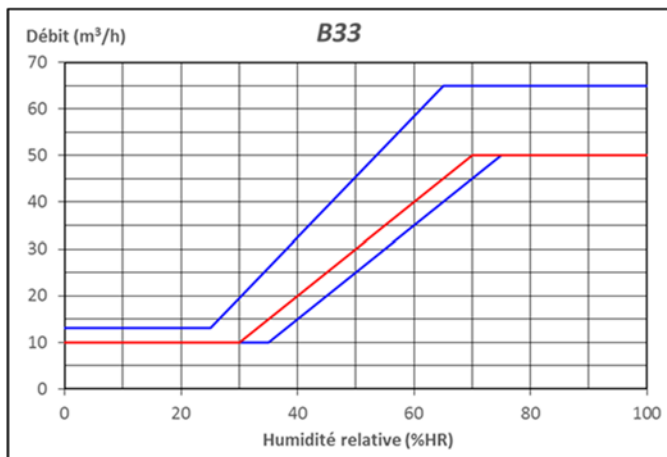
Figure 32 – B33 (10-50 m³/h, 30-70%HR)
