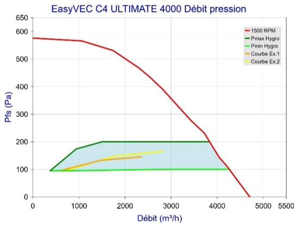
Figure 58 - EasyVEC C4 ULTIMATE 4000 (sans T.Flow Hygro+ /T.Flow Nano)
