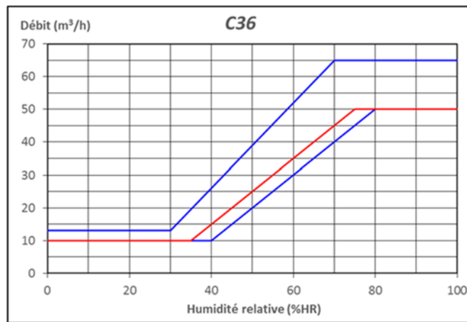
Figure 28 – C36 (10-50/90 m³/h, 35-75%HR)
