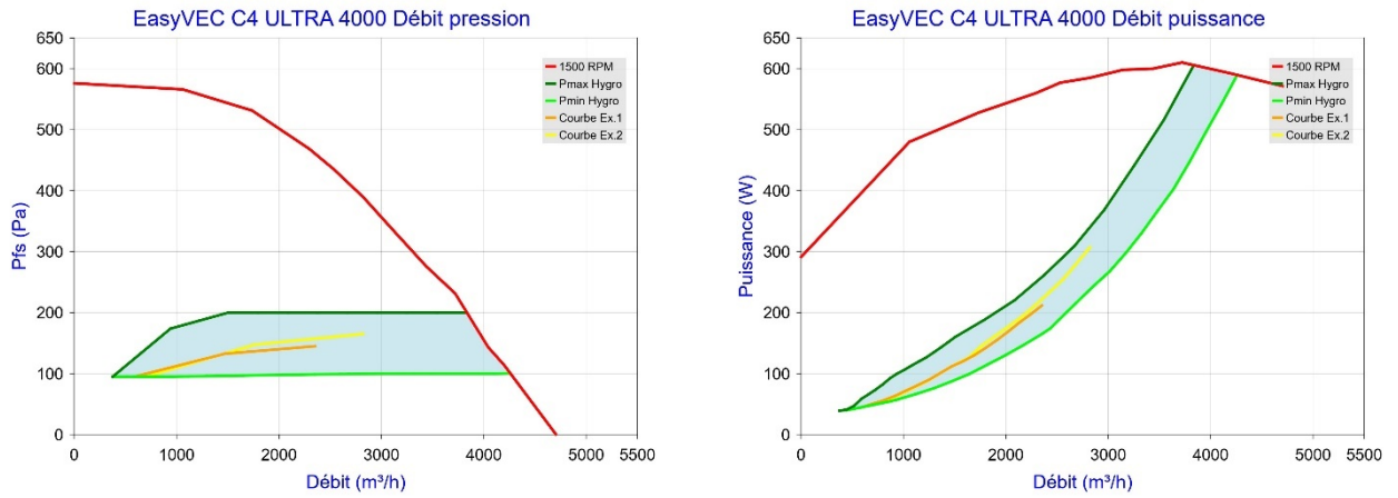
Figure 42 - EasyVEC C4 ULTRA 4000 (sans T.Flow Hygro+ /T.Flow Nano)
