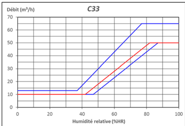
Figure 25 – C33 (10-50/105 m³/h, 42-82%HR)
