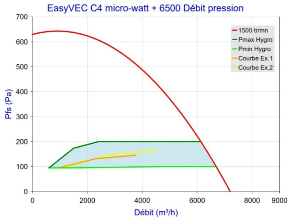
Figure 18 - EasyVEC C4 micro-watt + 6500 (sans T.Flow Hygro+ /T.Flow Nano)
