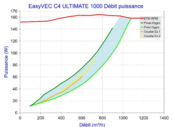
Figure 53 - EasyVEC C4 ULTIMATE 1000 (sans T.Flow Hygro+ /T.Flow Nano)
