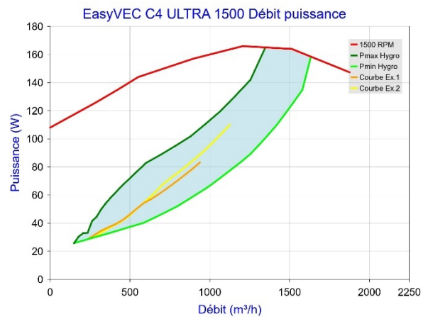
Figure 38 - EasyVEC C4 ULTRA 1500 (sans T.Flow Hygro+/T.Flow Nano)
