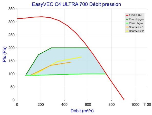
Figure 36 - EasyVEC C4 ULTRA 700 (sans T.Flow Hygro+/T.Flow Nano)
