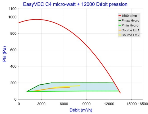
Figure 21 - EasyVEC C4 micro-watt + 12000 (sans T.Flow Hygro+ /T.Flow Nano)
