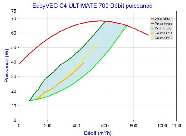
Figure 52 - EasyVEC C4 ULTIMATE 700 (sans T.Flow Hygro+ /T.Flow Nano)
