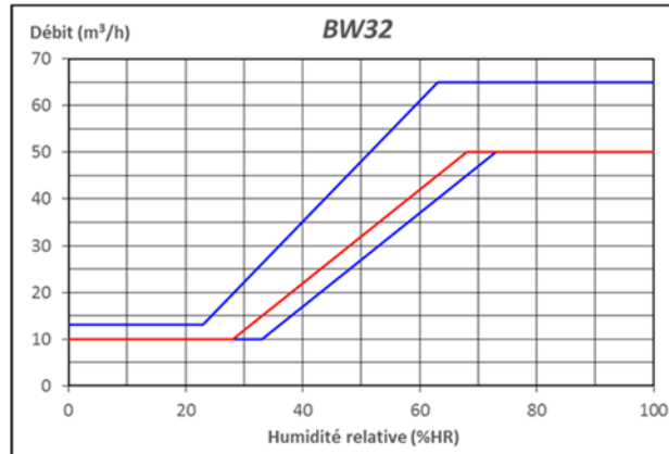
Figure 34 – BW32 (10-50/30 m³/h, 28-68%HR)
