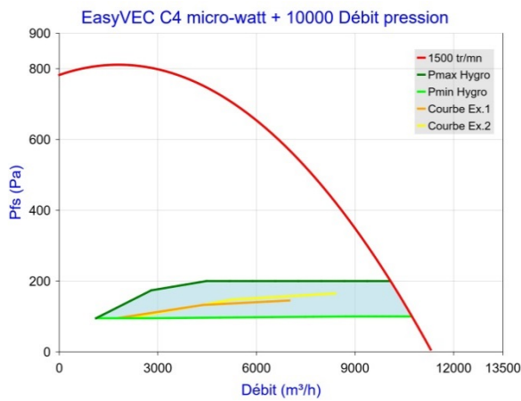
Figure 20 - EasyVEC C4 micro-watt + 10000 (sans T.Flow Hygro+ /T.Flow Nano)
