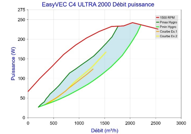
Figure 39 - EasyVEC C4 ULTRA 2000 (sans T.Flow Hygro+ / T.Flow Nano)
