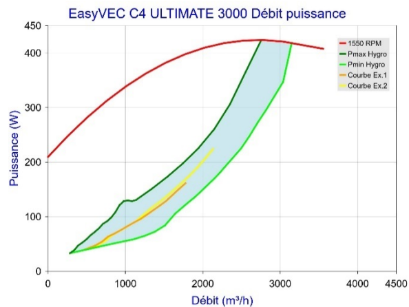
Figure 57 - EasyVEC C4 ULTIMATE 3000 (sans T.Flow Hygro+ / T.Flow Nano)
