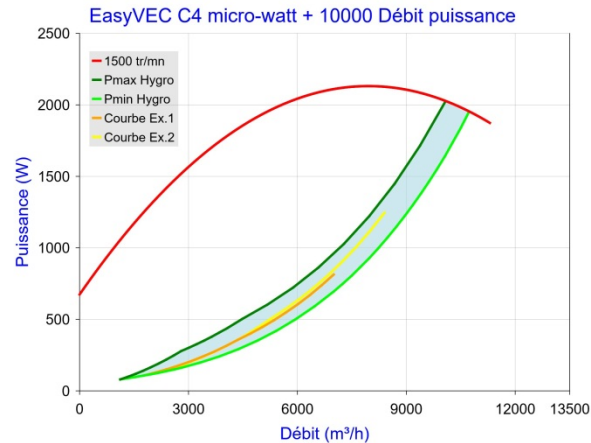
Figure 20 - EasyVEC C4 micro-watt + 10000 (sans T.Flow Hygro+ /T.Flow Nano)
