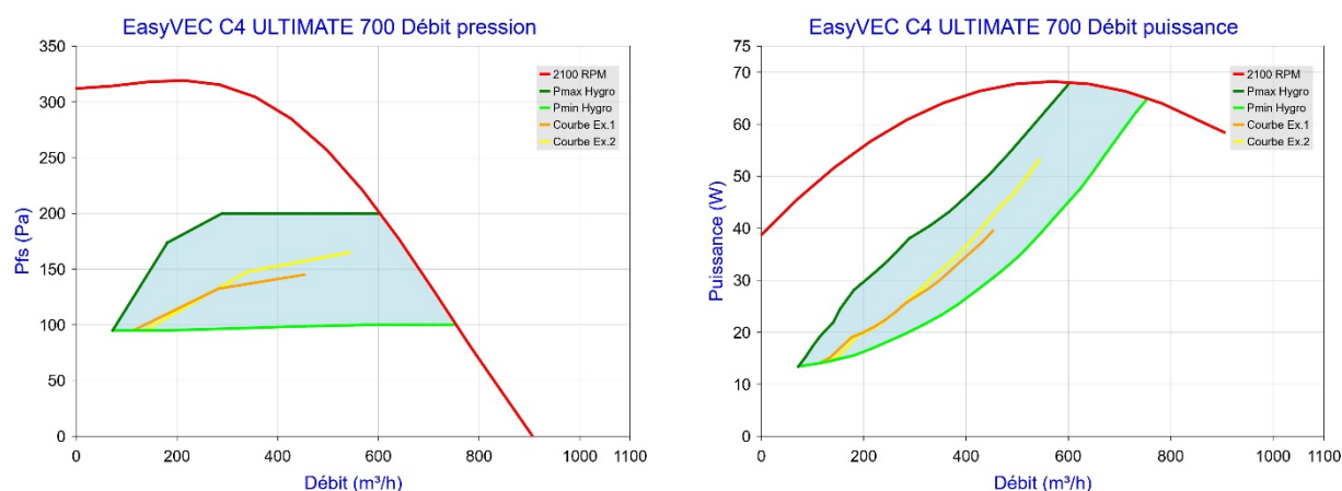
Figure 52 - EasyVEC C4 ULTIMATE 700 (sans T.Flow Hygro+ /T.Flow Nano)
