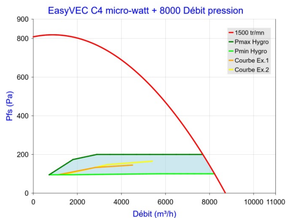
Figure 19 - EasyVEC C4 micro-watt + 8000 (sans T.Flow Hygro+ /T.Flow Nano)
