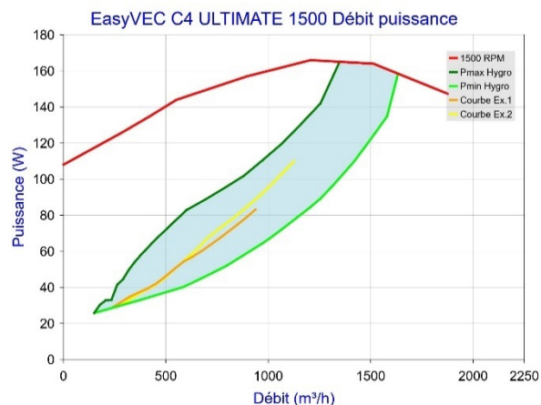
Figure 54 - EasyVEC C4 ULTIMATE 1500 (sans T.Flow Hygro+ / T.Flow Nano)
