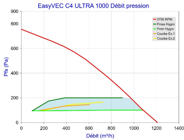
Figure 37 - EasyVEC C4 ULTRA 1000 (sans T.Flow Hygro+ / T.Flow Nano)
