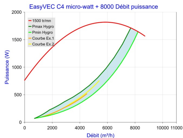
Figure 19 - EasyVEC C4 micro-watt + 8000 (sans T.Flow Hygro+ /T.Flow Nano)
