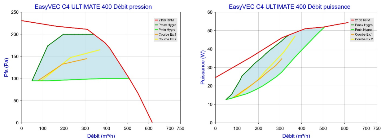
Figure 51 - EasyVEC C4 ULTIMATE 400 (sans T.Flow Hygro+ /T.Flow Nano)
