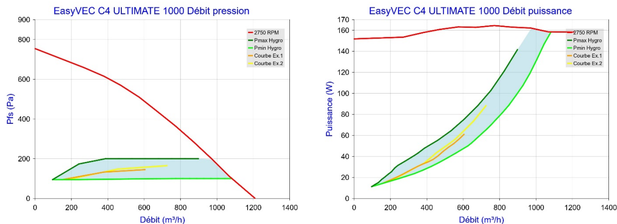
Figure 53 - EasyVEC C4 ULTIMATE 1000 (sans T.Flow Hygro+ /T.Flow Nano)
