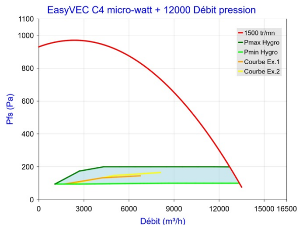
Figure 21 - EasyVEC C4 micro-watt + 12000 (sans T.Flow Hygro+ /T.Flow Nano)
