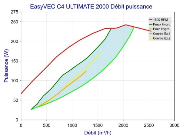
Figure 55 - EasyVEC C4 ULTIMATE 2000 (sans T.Flow Hygro+ / T.Flow Nano)
