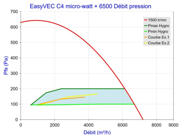
Figure 18 - EasyVEC C4 micro-watt + 6500 (sans T.Flow Hygro+ /T.Flow Nano)
