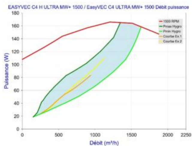
Figure 85 - EasyVEC C4 (H) ULTRA MW+ 1500 (sans T.Flow Hygro+/T.Flow Nano)
