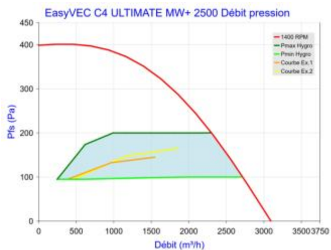
Figure 103 - EasyVEC C4 ULTIMATE MW+ 2500 (sans T.Flow Hygro+/T.Flow Nano)
