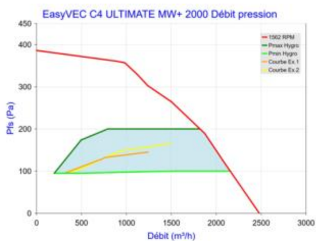
Figure 102- EasyVEC C4 ULTIMATE MW+ 2000 (sans T.Flow Hygro+/T.Flow Nano)
