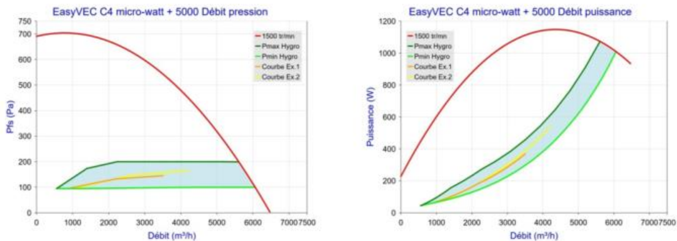
Figure 64 - EasyVEC C4 micro-watt + 5000 (sans T.Flow Hygro+/T.Flow Nano)
