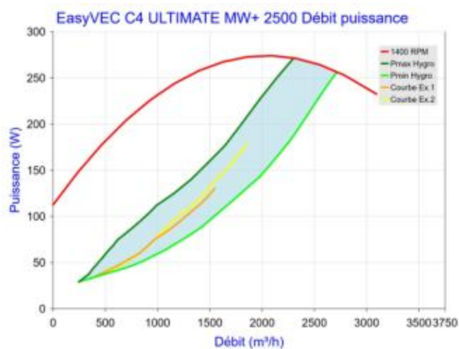
Figure 103 - EasyVEC C4 ULTIMATE MW+ 2500 (sans T.Flow Hygro+/T.Flow Nano)
