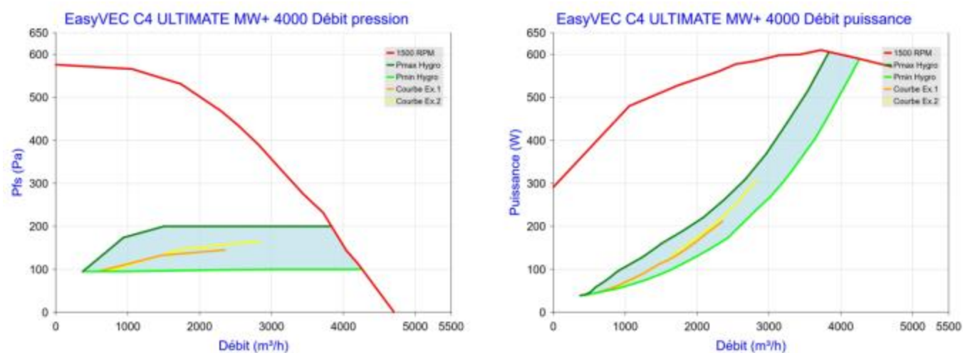
Figure 105 - EasyVEC C4 ULTIMATE MW+ 4000 (sans T.Flow Hygro+/T.Flow Nano)
