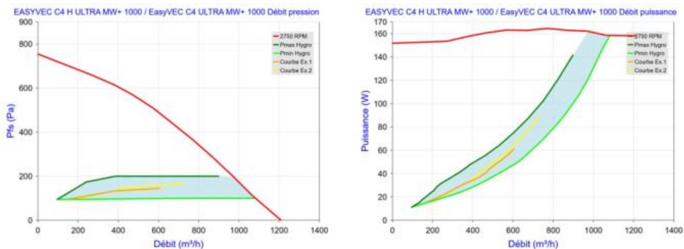
Figure 84 - EasyVEC C4 (H) ULTRA MW+ 1000 (sans T.Flow Hygro+/T.Flow Nano)
