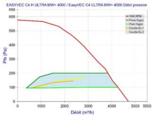
Figure 89 - EasyVEC C4 (H) ULTRA MW+ 4000 (sans T.Flow Hygro+/T.Flow Nano)
