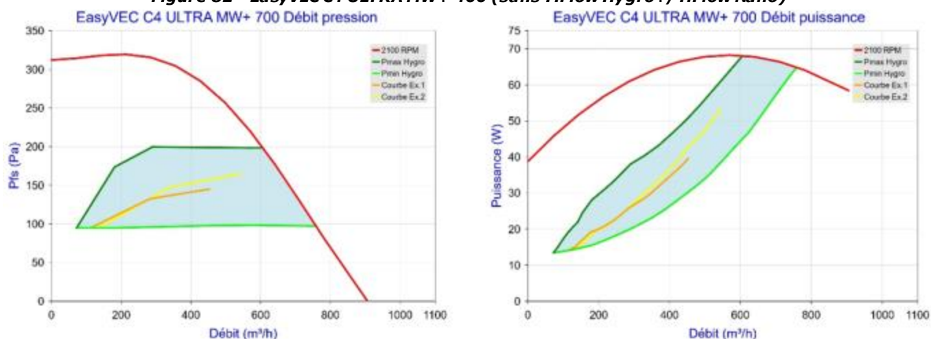
Figure 83 - EasyVEC C4 ULTRA MW+ 700 (sans T.Flow Hygro+/T.Flow Nano)
