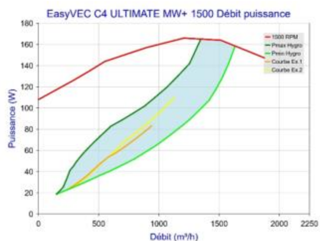
Figure 101 - EasyVEC C4 ULTIMATE MW+ 1500 (sans T.Flow Hygro+/T.Flow Nano)
