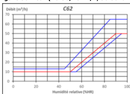
Figure 31 – C62 (10-50/90 m³/h, 50-90%HR)
