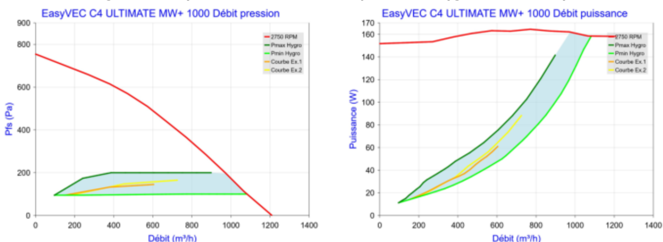
Figure 100 - EasyVEC C4 ULTIMATE MW+ 1000 (sans T.Flow Hygro+/T.Flow Nano)
