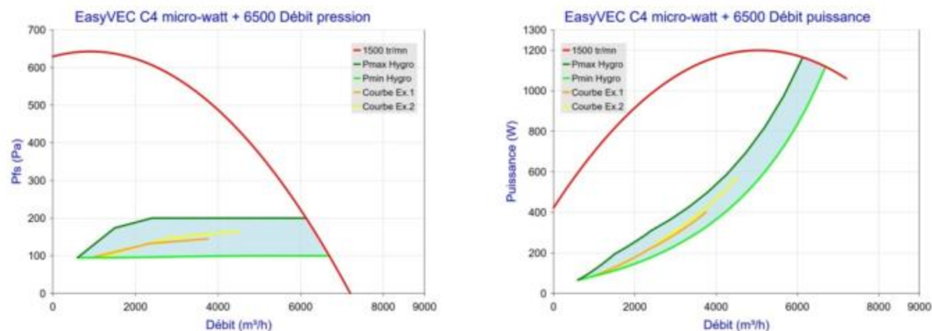
Figure 65 - EasyVEC C4 micro-watt + 6500 (sans T.Flow Hygro+/T.Flow Nano)
