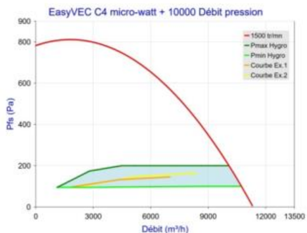
Figure 67 - EasyVEC C4 micro-watt + 10000 (sans T.Flow Hygro+/T.Flow Nano)
