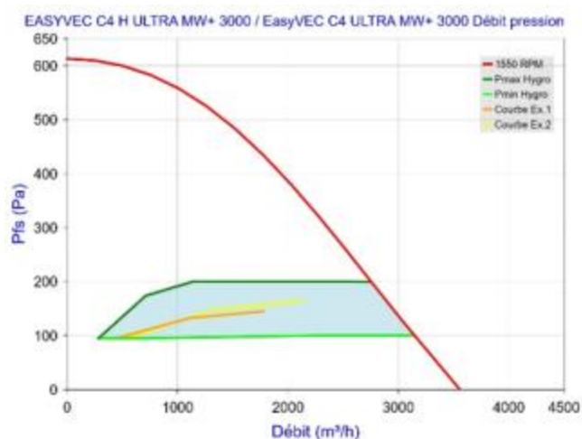
Figure 88 - EasyVEC C4 (H) ULTRA MW+ 3000 (sans T.Flow Hygro+/T.Flow Nano)
