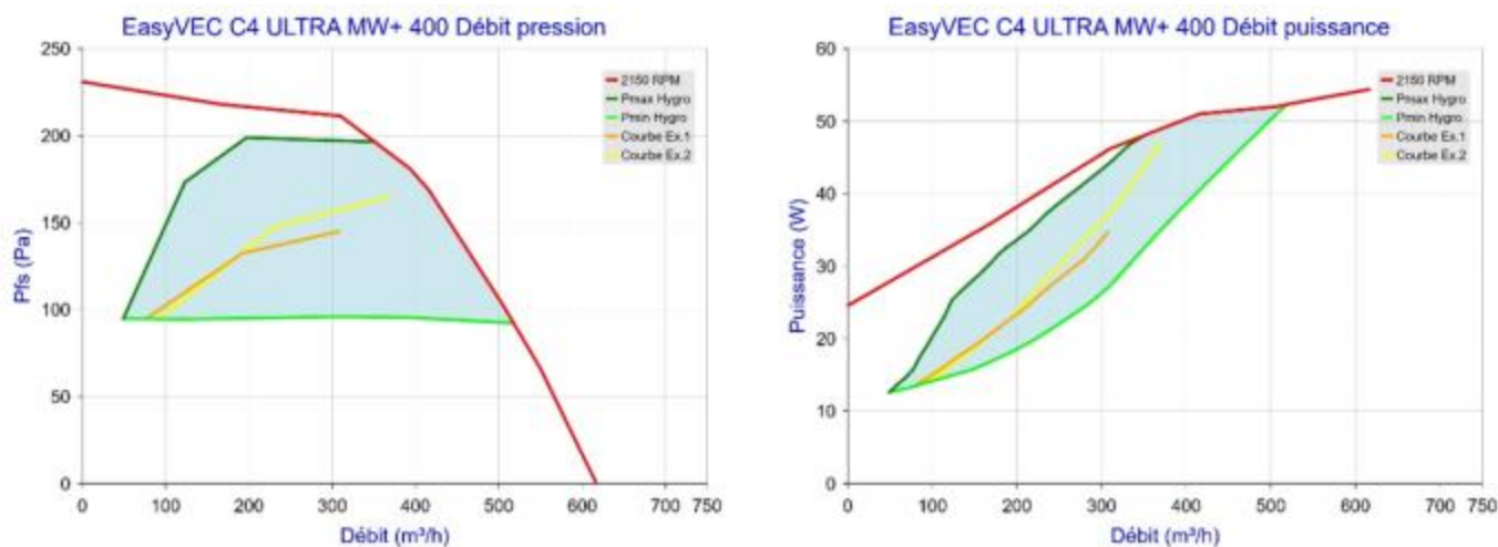
Figure 82 - EasyVEC C4 ULTRA MW+ 400 (sans T.Flow Hygro+/T.Flow Nano)
