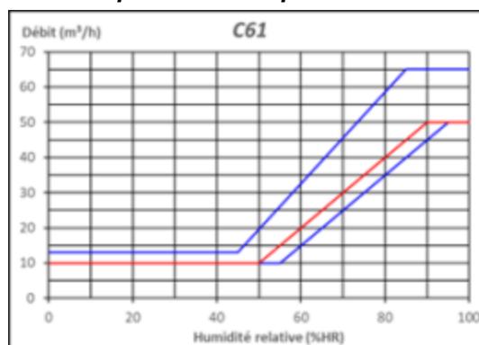
Figure 30 – C61 (10-50/75 m³/h, 50-90%HR)
