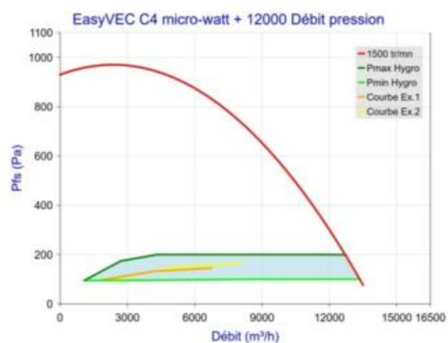
Figure 68 - EasyVEC C4 micro-watt + 12000 (sans T.Flow Hygro+/T.Flow Nano)
