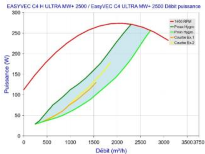
Figure 87 - EasyVEC C4 (H) ULTRA MW+ 2500 (sans T.Flow Hygro+/T.Flow Nano)
