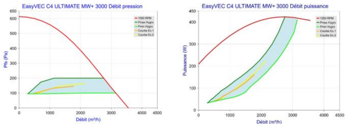
Figure 104 - EasyVEC C4 ULTIMATE MW+ 3000 (sans T.Flow Hygro+/T.Flow Nano)
