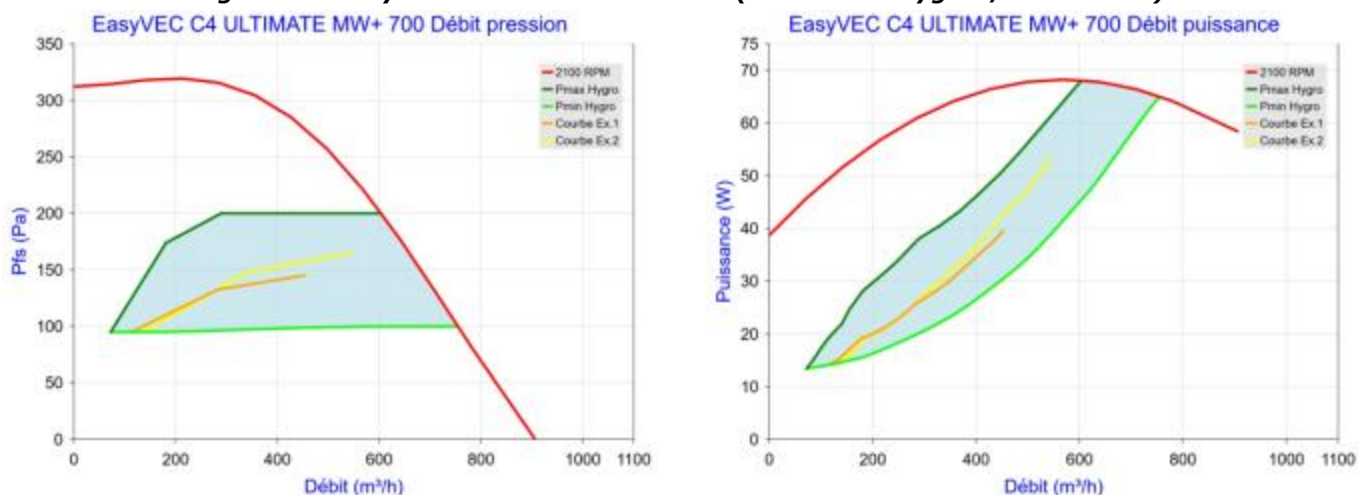
Figure 99 - EasyVEC C4 ULTIMATE MW+ 700 (sans T.Flow Hygro+/T.Flow Nano)
