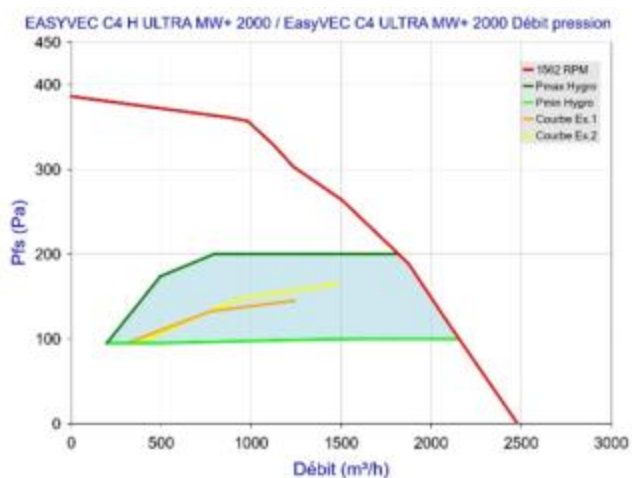
Figure 86 - EasyVEC C4 (H) ULTRA MW+ 2000 (sans T.Flow Hygro+/T.Flow Nano)
