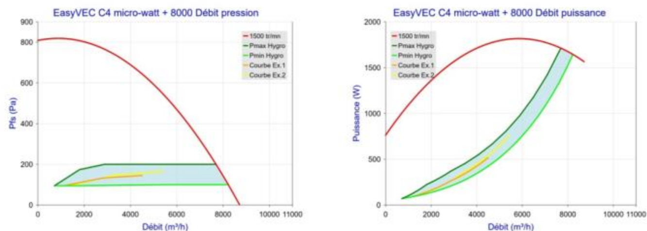
Figure 66 - EasyVEC C4 micro-watt + 8000 (sans T.Flow Hygro+/T.Flow Nano)
