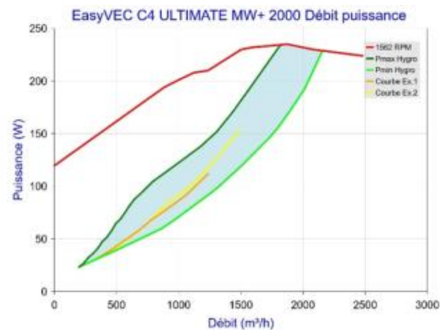
Figure 102- EasyVEC C4 ULTIMATE MW+ 2000 (sans T.Flow Hygro+/T.Flow Nano)
