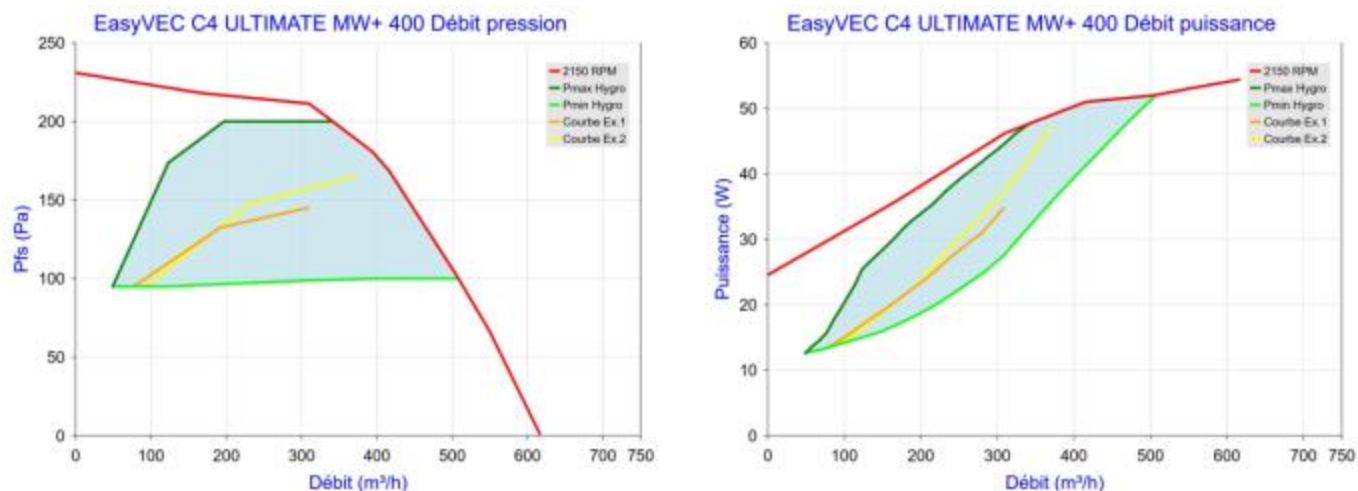
Figure 98 - EasyVEC C4 ULTIMATE MW+ 400 (sans T.Flow Hygro+/T.Flow Nano)
