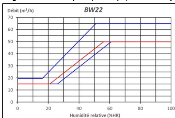
Figure 37 – BW22 (15-50/50 m³/h, 21-56%HR)
