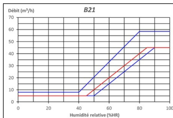
Figure 33 - B21 (5-45 m³/h, 45-85%HR)
