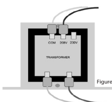
Figure 1: Transformer Wiring for 230V
