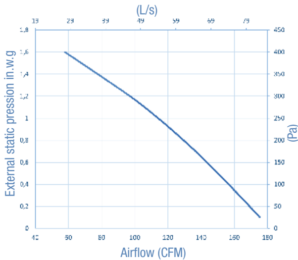
EK150-TF Ventilation Performance
