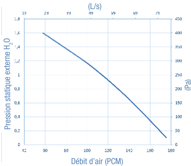
EK150-TF Performance de ventilation
