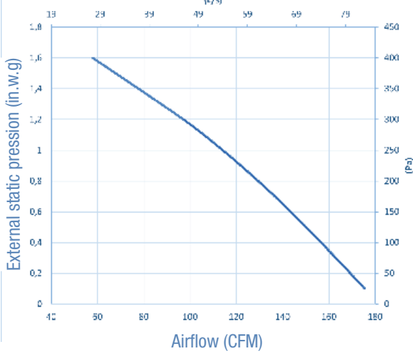
EK150-TQG Ventilation Performance
