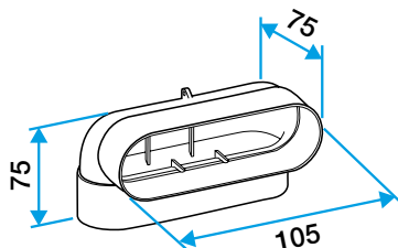
Coude vertical 90°
