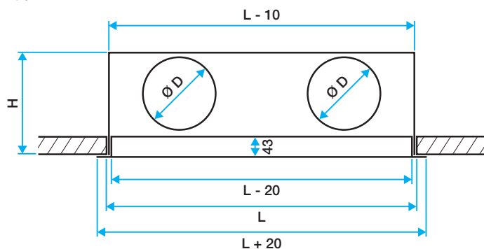
Plénum LINED
