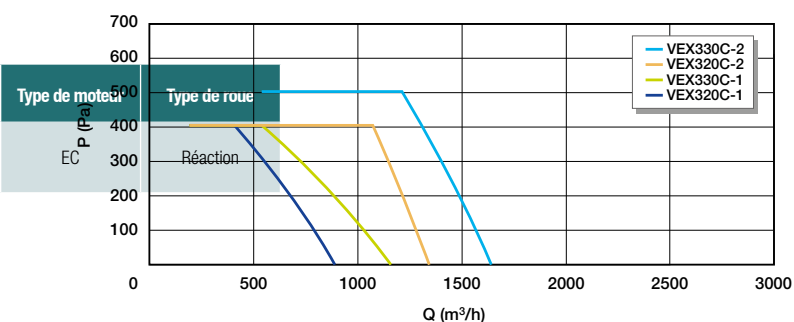
Aeraulic characteristics VEX300C
