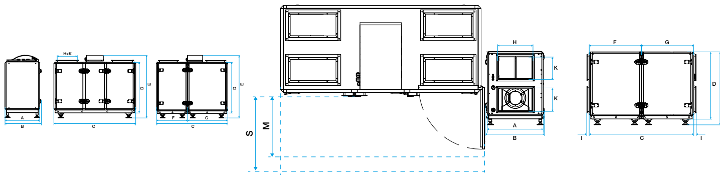
Dimensions VEX700T
