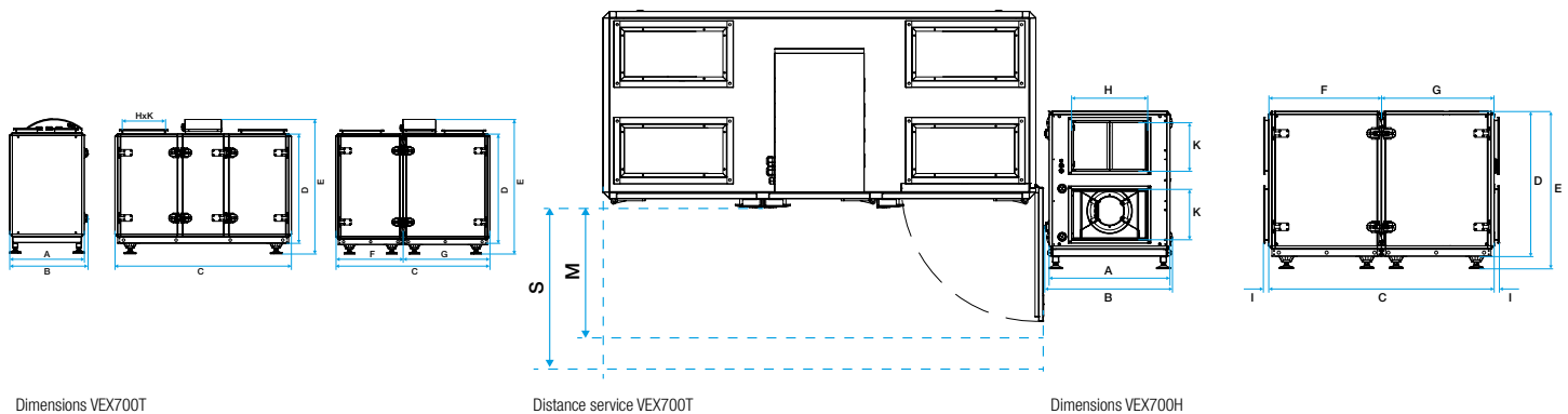
Dimensions VEX700T
