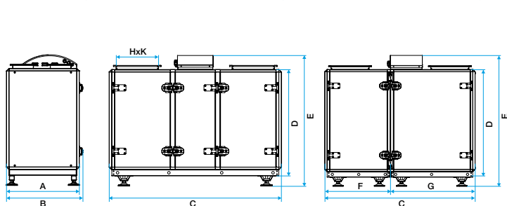
Dimensions VEX700T
